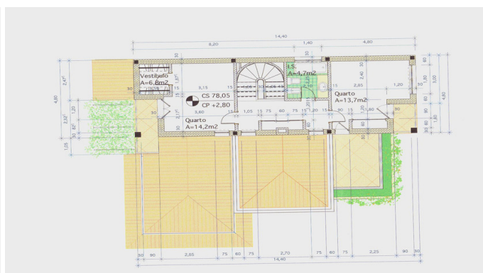
PISO 1.0 A=60,0m 2
